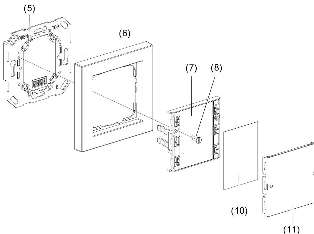
picture 3: Device fitting using the example of a push button 3 comfort 1-gang
