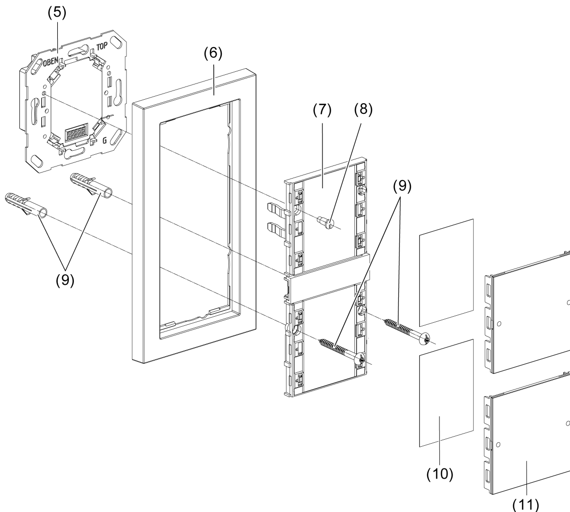
picture 4: Device fitting using the example of a push button 3 comfort 2-gang (with frame and without central bar)
