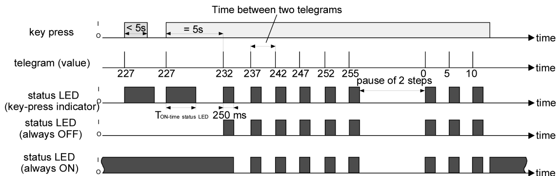
picture 16: Example of value adjustment with value range overflow
