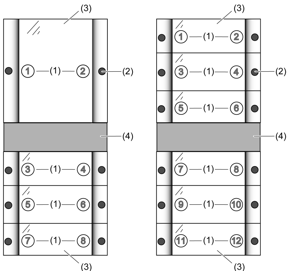
picture 2: Device components Pushbutton sensors 3 comfort - 4gang and 6gang variants
