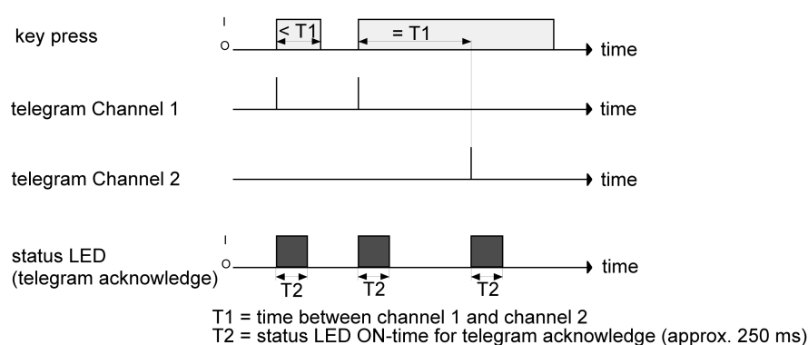
picture 18: Example for operation concept "Channel 1 and channel 2"
