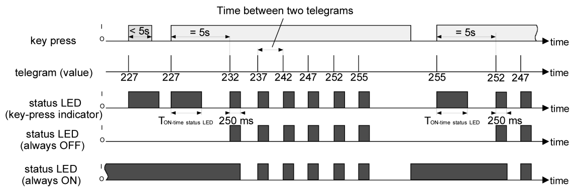
picture 15: Example of value adjustment without value range overflow
