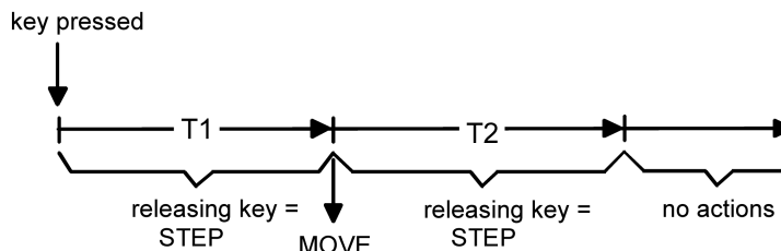
picture 14: Operation concept "long – short or short"
