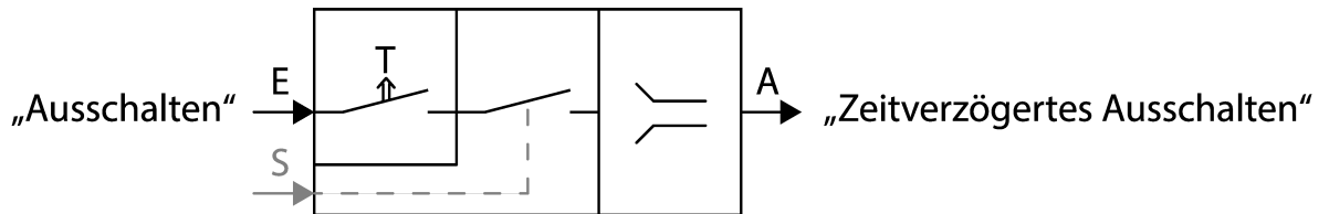
Figure 22: "Delayed switch-off" diagram
