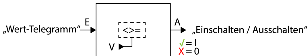
Figure 26: "Status indication reference value" diagram
