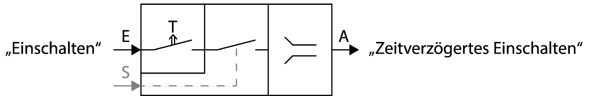
Figure 21: "Delayed switch-on" diagram
