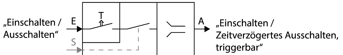
Figure 24: "Staircase function" diagram
